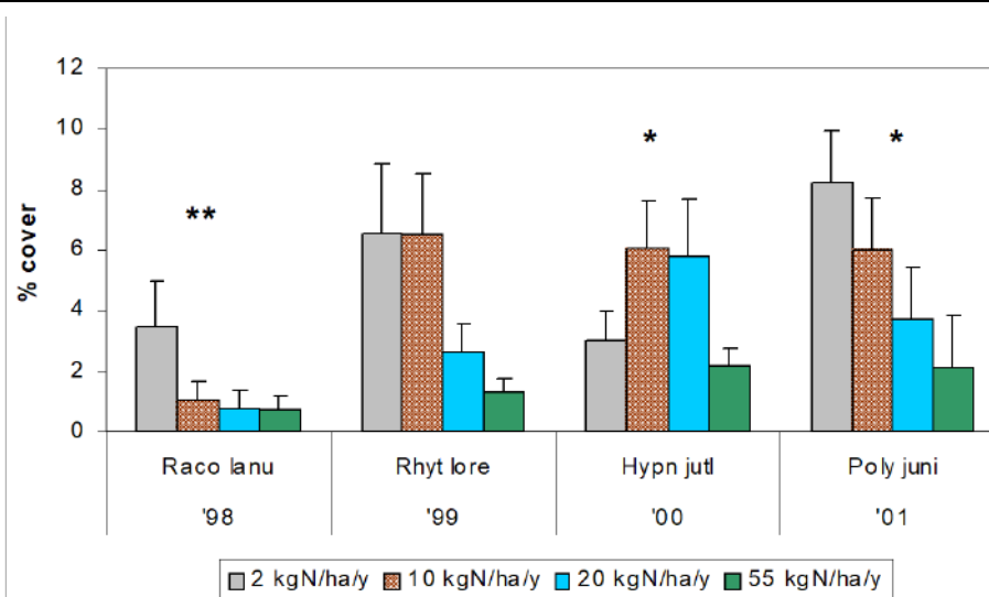
Figure 7.7. Cover of moss species in Nardus stricta grassland mesocosms, exposed since 1997 to four N treatments (2, 10, 20, and 55 kg N ha -1 yr -1 ; from left to right). The mosses are Racomitrium lanuginosum , Rhytidiadelphus loreus , Hypnum jutlandicum and Polytrichum juniperinum .
