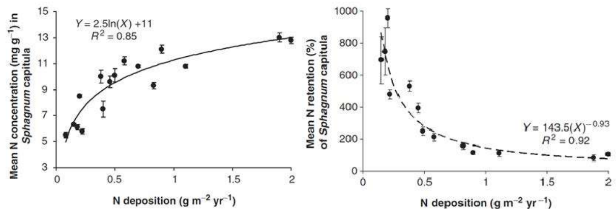
Figure 6.7 a) Trend of mean (± SE) nitrogen (N) concentration in Sphagnum capitula along the gradient of atmospheric N and b) Mean (± SE) N retention by Sphagnum capitula along the gradient in atmospheric N deposition. To convert g m -2 to kg ha -1 multiply by 10. N retention was calculated as the ratio between capitulum N concentration per square metre and atmospheric N deposition.
