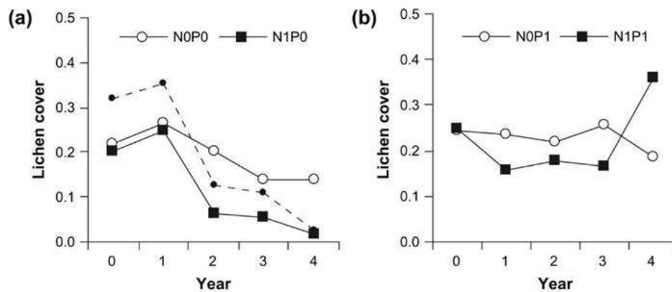
Figure 8.5. Effect of factorial combinations of N and P additions on the cover of lichens in an upland Calluna vulgaris heath (background N deposition of 16.4 \text{ kg N ha}^{-1} \text{ yr}^{-1} ). N0 = 0 \text{ kg N ha}^{-1} \text{ yr}^{-1} , N1 = 20 \text{ kg N ha}^{-1} \text{ yr}^{-1} , P0 = 0 \text{ kg P ha}^{-1} \text{ yr}^{-1} and P1 = 5 \text{ kg P ha}^{-1} \text{ yr}^{-1} . The dotted line in Figure (a) indicates a separate N addition of 10 \text{ kg N ha}^{-1} \text{ yr}^{-1} . The decline in Lichen cover in the control (N0P0) reflects the increased growth of the Calluna canopy.
