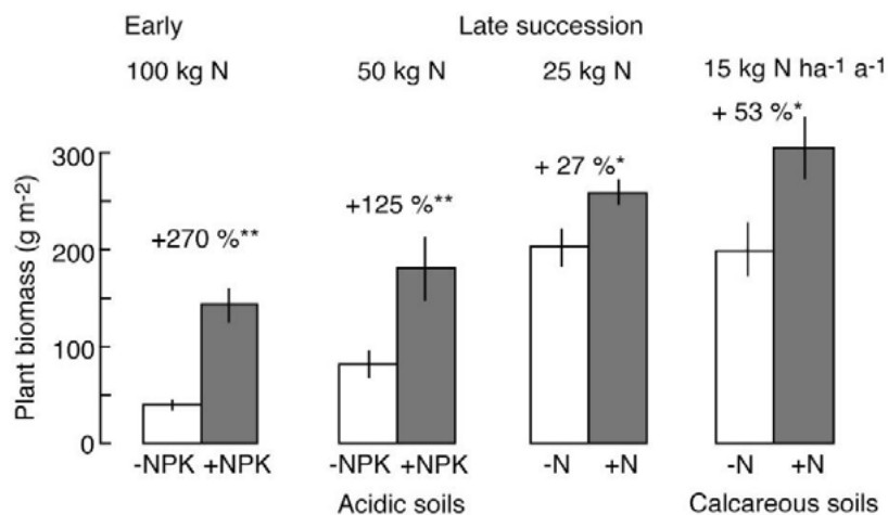
Figure 7.8. Responses of vegetation of high elevation (> 2450 m) grassland and glacier foreland (most left) to two to four years of nutrient addition in early and late successional habitats, control plots are shown as -NPK or -N.
